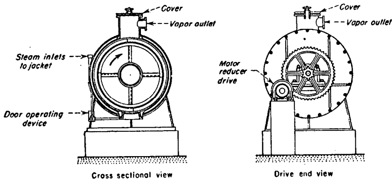
FIG 10 - A TYPICAL VACUUM ROTARY DRYER (Blaw-Knox Co)
